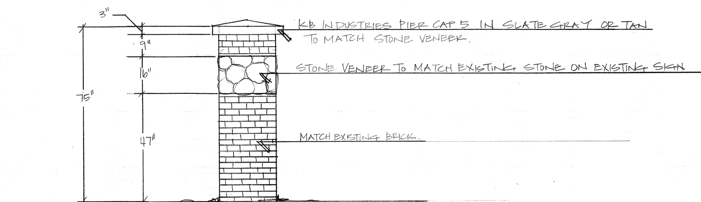
DESIGN CONCEPT NEW PILASTERS NOT TO SCALE
